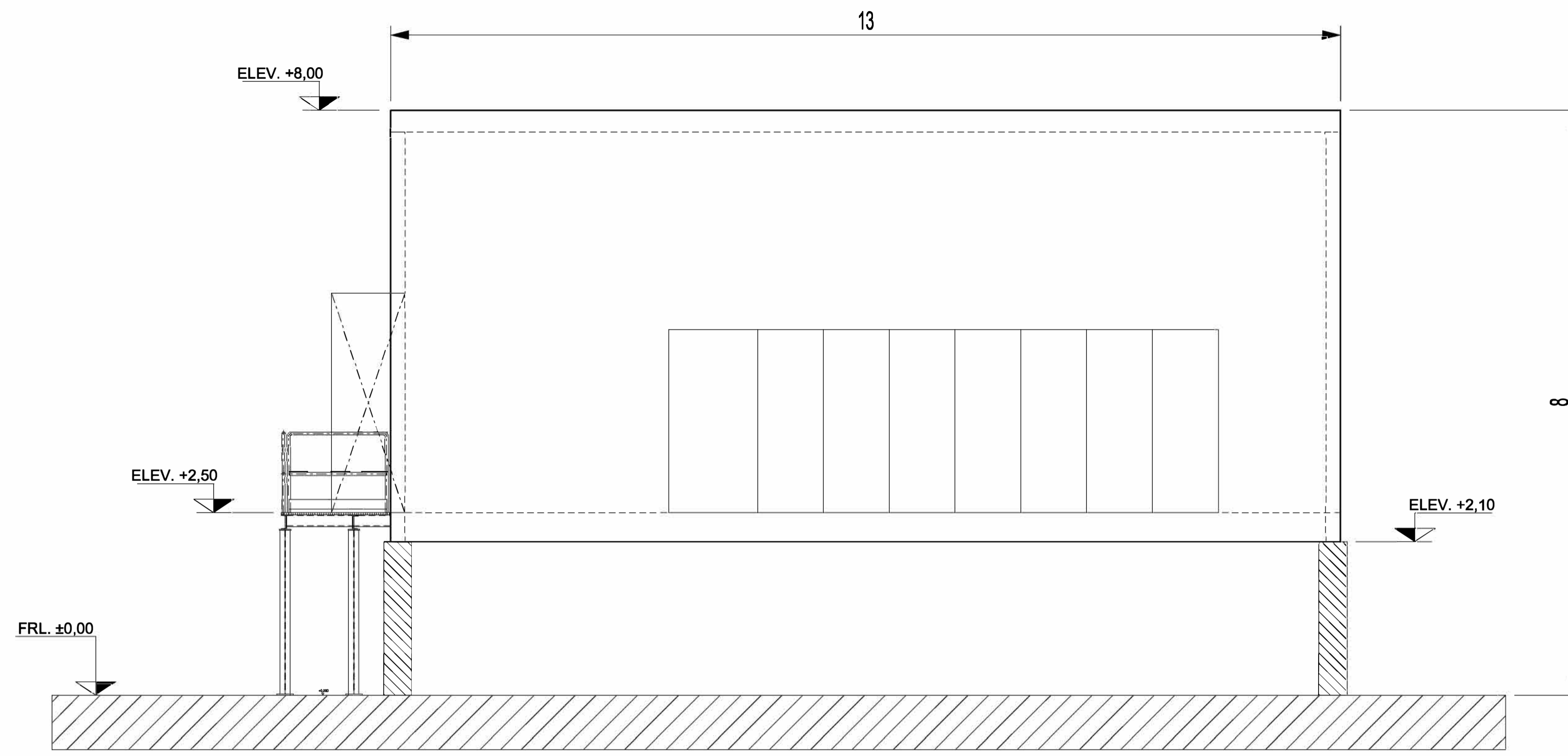
FRONT VIEW
