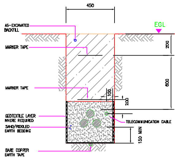
3 No. 33kV CABLES IN TREFOIL FORMATION SCALE 1:20
