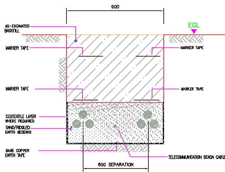
2 SETS OF 3 No. 33kV CABLES IN TREFOIL FORMATION SCALE 1:20
