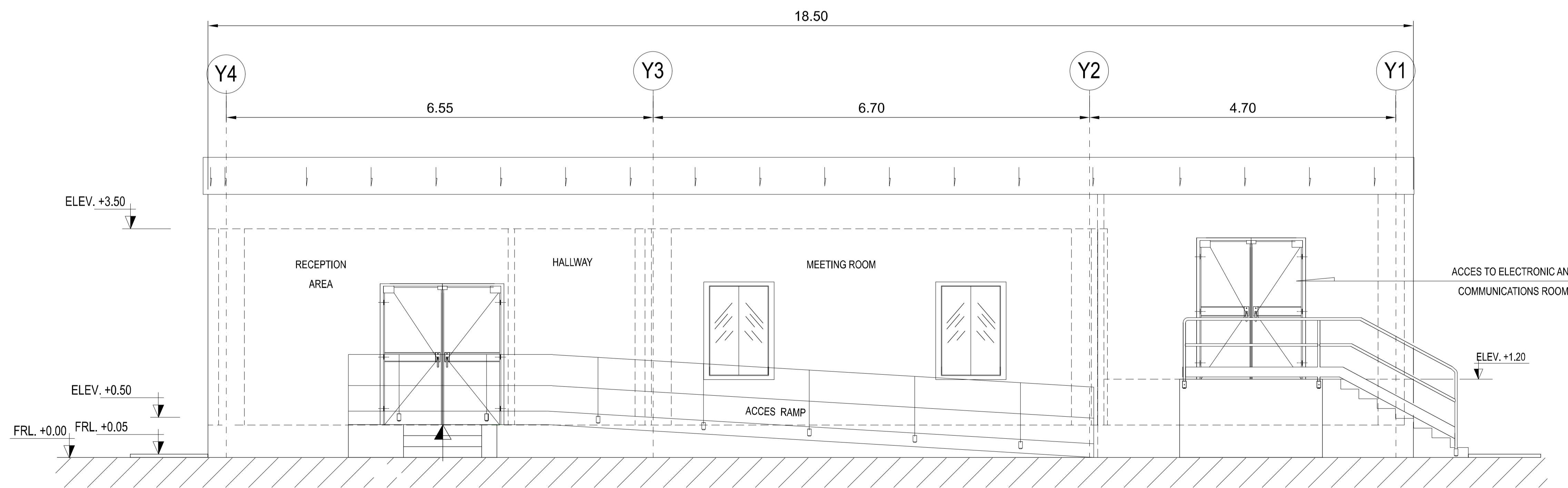
SECTION "B-B"
